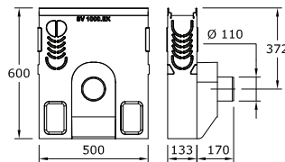
MEADRAIN Catch basin 1000.EK (with trap Ø 110 or Ø 160mm)
