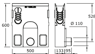
MEADRAIN Catch basin SV 1000.EK (with connection Ø 110 or Ø 160mm)
