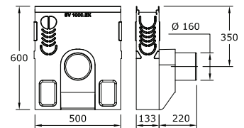
MEADRAIN Catch basin 1000.EK (with trap Ø 110 or Ø 160mm)
