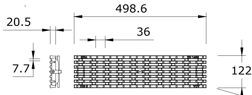
SV 1000 ADA longitudinal ductile iron grating 36/7.7 with CLIPFIX, loading class E600**
