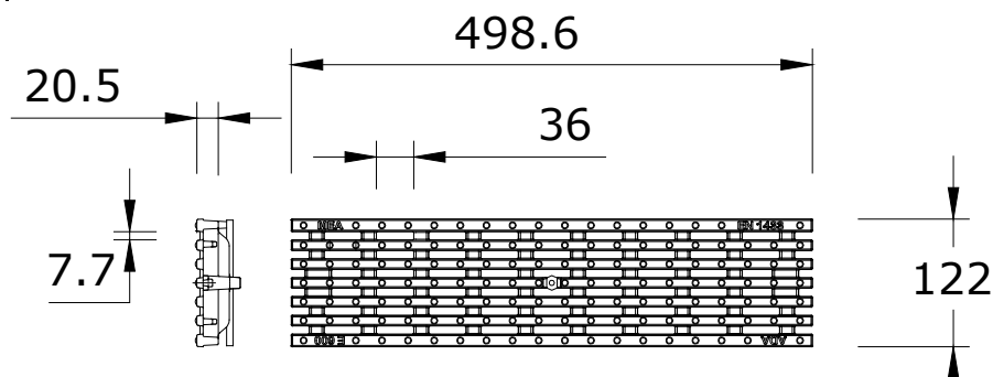
EN 1000 ADA longitudinal ductile iron grating 36/7.7 with PROFIX, loading class E600**
