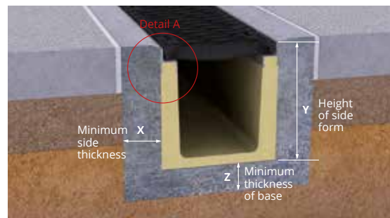
Detail A Channel with edge 3-5mm from the edge
