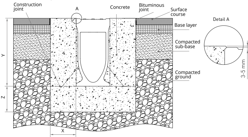
D400 - E600 - F900 Transversal to the traffic direction
