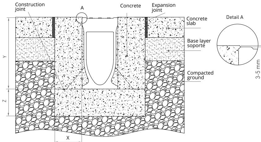
D400 - E600 - F900 Longitudinal to the traffic direction
